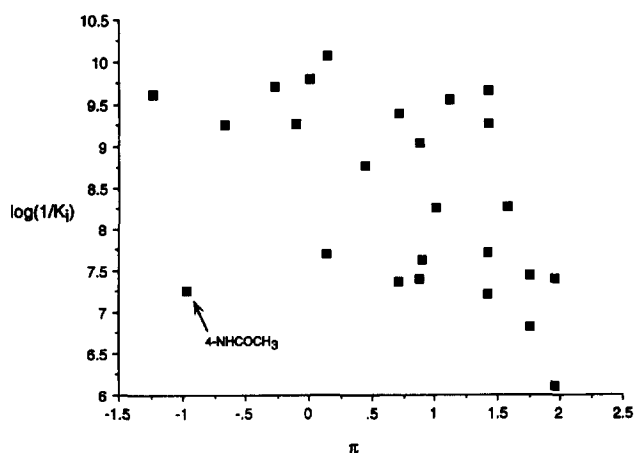
Figure 1. Potency at CCK-B receptors vs \pi of phenyl substituents.
