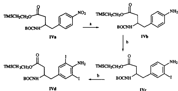
Scheme 2. (a) \text{Pd}(\text{OH})_2/\text{C} ; (b) Chloramine T, NaI, HOAc.
