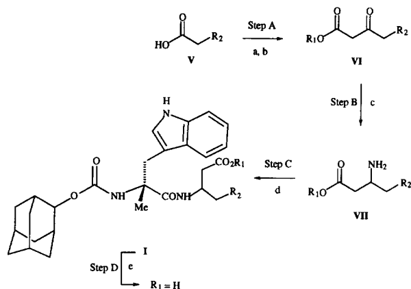
Scheme 4. Method B. (a) CDI, 0 °C; (b) (R_1\text{OCOCH}_2\text{CO}_2^-) \text{Mg}^{2+} , \text{CH}_3\text{CN} , 25 °C; (c) \text{NH}_4\text{OAc}/\text{MeOH} , \text{NaBH}_3\text{CN} , 3 Å sieves; (d) 2-Adoc- \alpha -Me-Trp-OH, DCC, HOBT; (e) \text{LiOH} , \text{H}_2\text{O}/\text{dioxane} .
