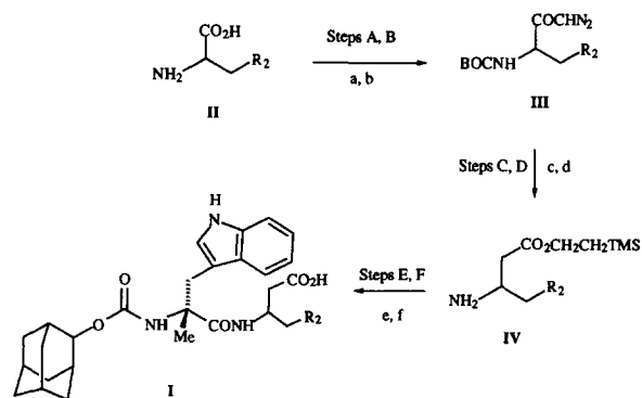
Scheme 1. Method A. (a) (\text{BOC})_2\text{O} , \text{NaHCO}_3 , aq dioxane; (b) i. i\text{-BuOCOC} , N -Me-morpholine, THF; ii. \text{CH}_2\text{N}_2 , \text{Et}_2\text{O} ; (c) \text{PhCO}_2\text{Ag} , \text{NEt}_3 , \text{TMSCH}_2\text{CH}_2\text{OH} ; (d) p -TSA; (e) 2-Adoc- R - \alpha -Me-Trp-OH, DCC, HOBt; (f) TBAF, THF.
