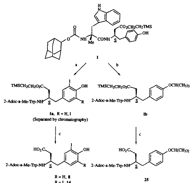
Scheme 3. (a) Chloramine T, NaI, MeCN; (b) \text{ICH}(\text{CH}_3)_2 , 2-butanone, \text{K}_2\text{CO}_3 ; (c) TBAF, THF.
