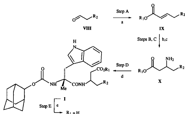
Scheme 5. Method C. (a) R_2\text{OCOCHPhPPh}_3 , THF, 25 °C; (b) \text{PhNH}_2 , \text{C} , \text{EtOH} , \Delta ; (c) 10% Pd/C, \text{H}_2 ; (d) 2-Adoc- \alpha -Me-Trp-OH; DCC, HOBT, DMAP; (e) \text{LiOH} , \text{H}_2\text{O}/\text{dioxane} .
